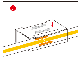
3. Put the COB light strip inside the crystal connector and press the iron piece down.
